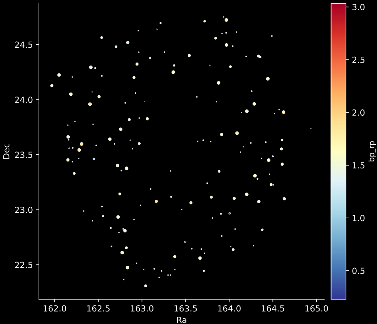
APOGEE DR17 Field: [K2_C13_171-20_btx] Stars: 156
