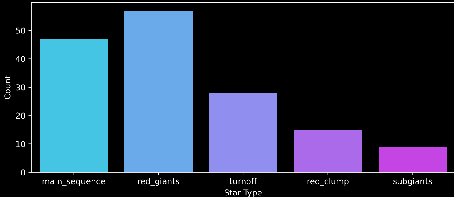
APOGEE DR17 Field: [K2_C13_171-20_btx] Count plot of Star Type
