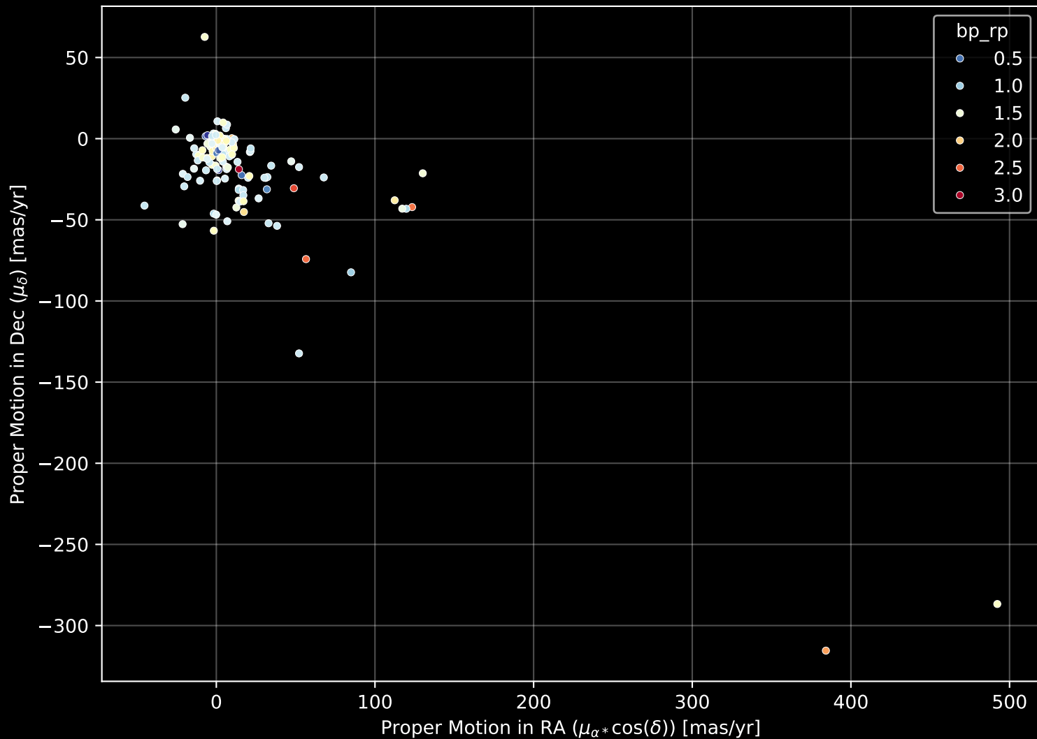
APOGEE DR17 Field: [K2_C13_171-20_btx] Proper Motion Diagram (n= 156)
