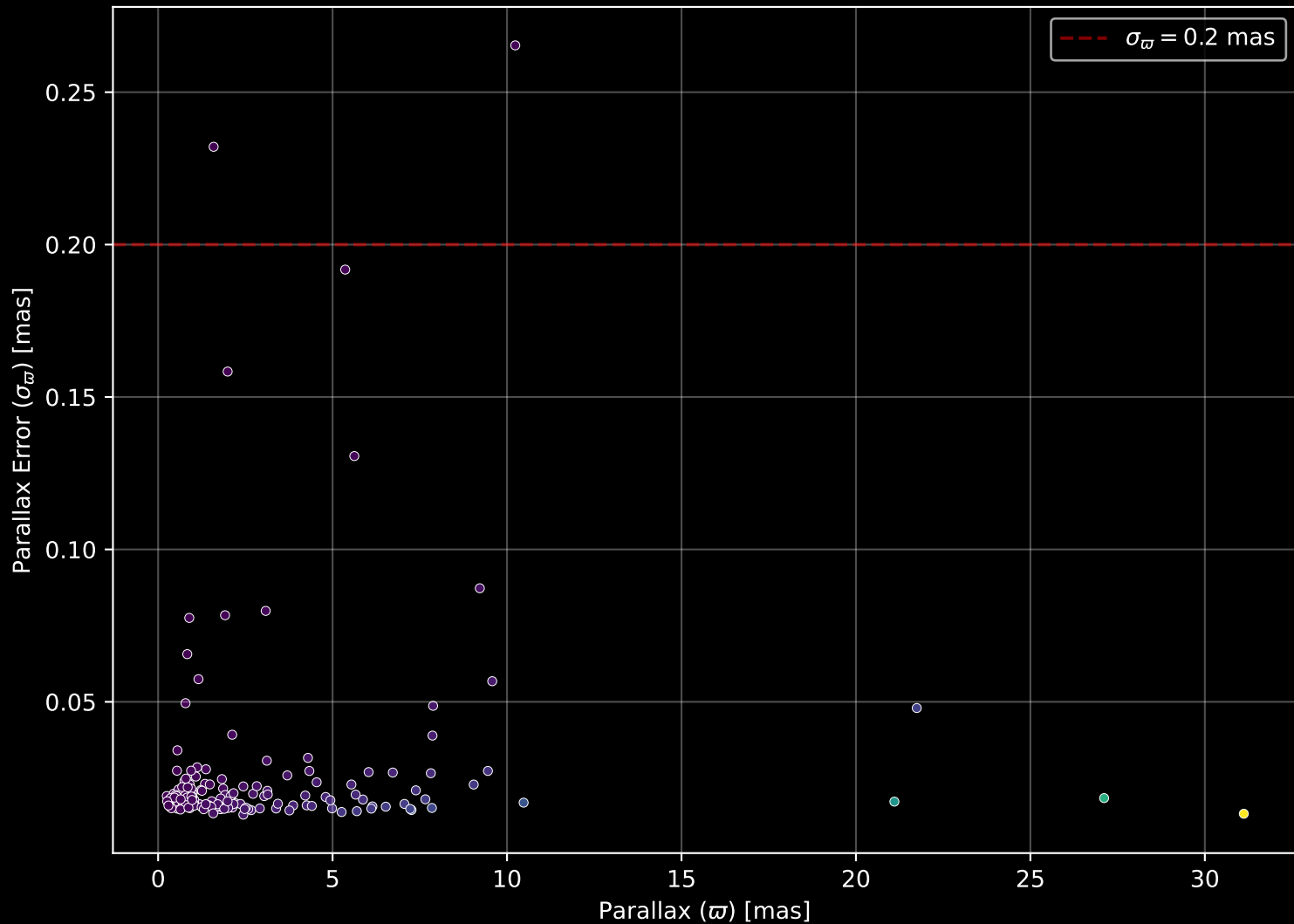
APOGEE DR17 Field: [K2_C13_171-20_btx] Parallax Quality (n= 156)
