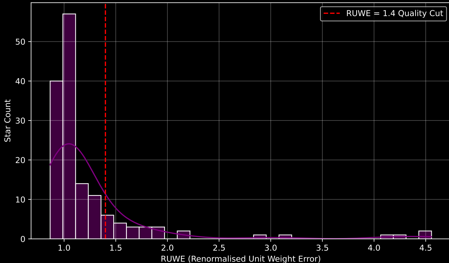
GAPOGEE DR17 Field [K2_C13_171-20_btx] RUWE Distribution (n= 149)
