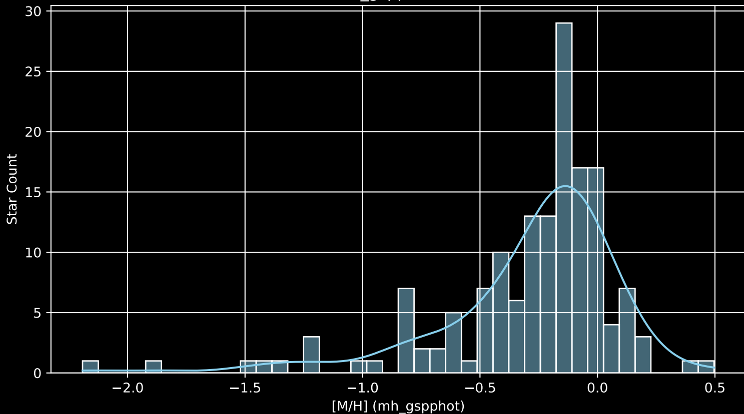
APOGEE DR17 Field: [K2_C13_171-20_btx [M/H] (mh_gspphot) (n= 155)
